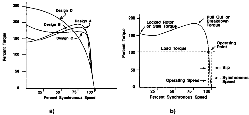
Figure 6-11—Typical speed-torque curves for NEMA design motors
