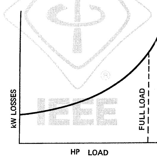
Figure 3-2—Motor losses
