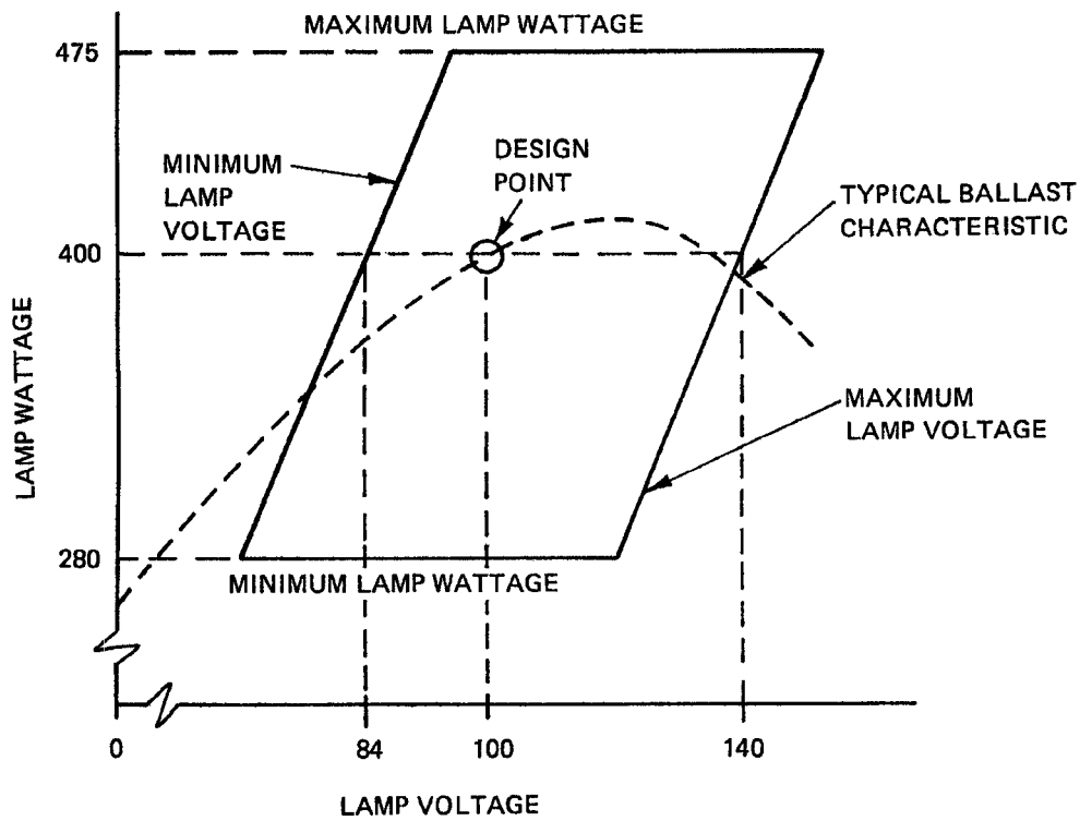
Figure 7-6—Trapezoid diagram for the 400 W HPS lamp
