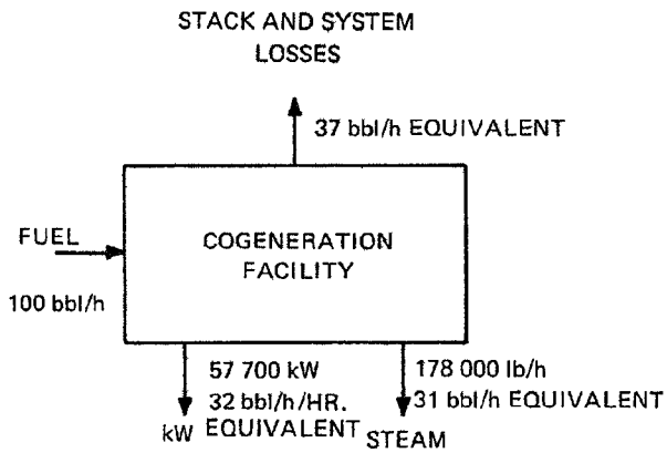
Figure 8-5—Cogeneration fuel-saving potential (unit comparison)
