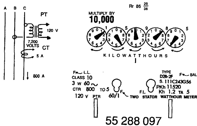
Figure 6-7—Electromechanical kilowatt-hour meter
