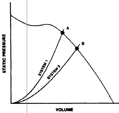
(c) Operating points using constant speed fan
