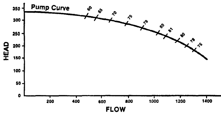
(a) Pump curve and efficiency data
