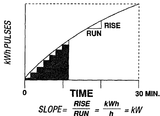
Figure 6-4—Demand curve
