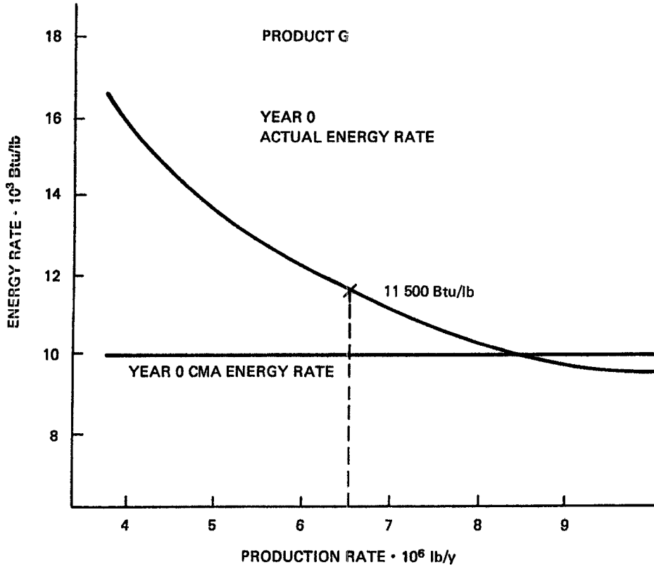
Figure 2-4—Actual and CMA energy rate versus production rate
