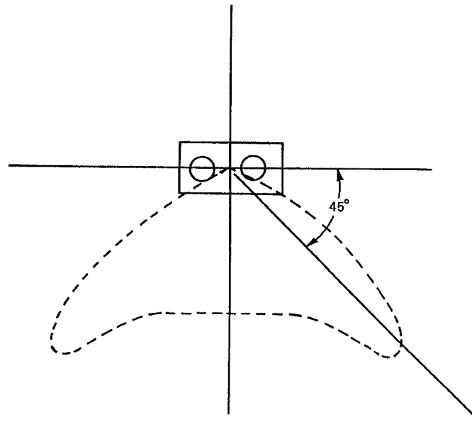
Figure 7-8—Batwing distribution
