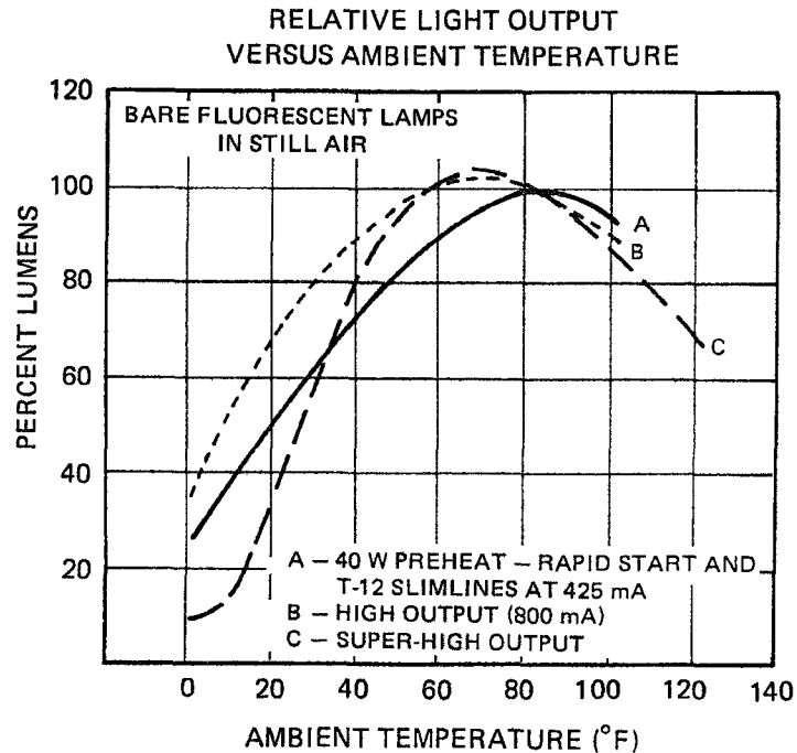
Figure 7-3—Relationship of lumens versus ambient temperature
