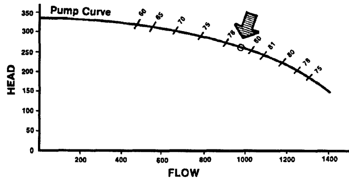
(c) Measure flow with valve fully open
