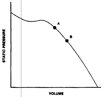
(a) Fan performance curve
