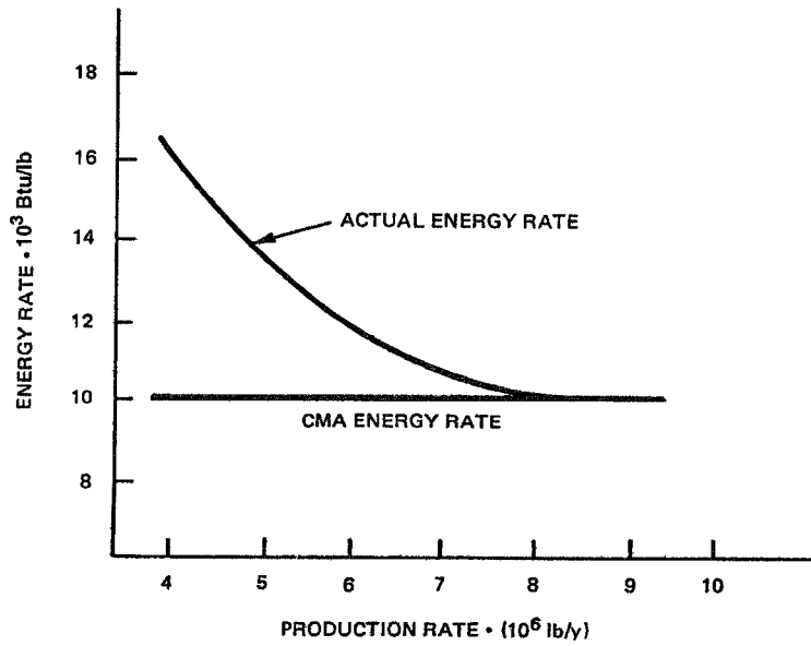
Figure 2-2—Change in production
