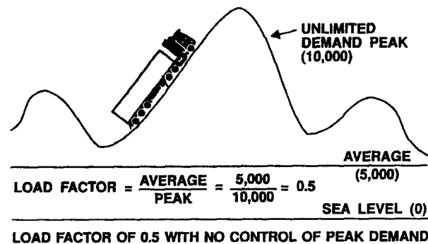
Figure 6-5—Load factor without peak demand control
