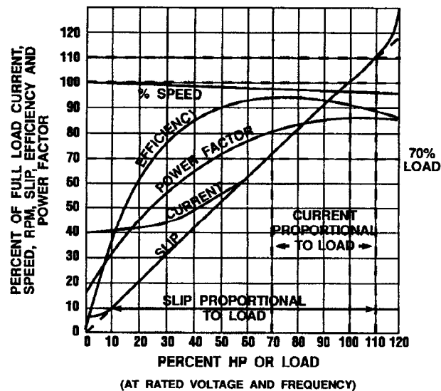
Figure 6-12—Typical NEMA Design B induction motor curve
