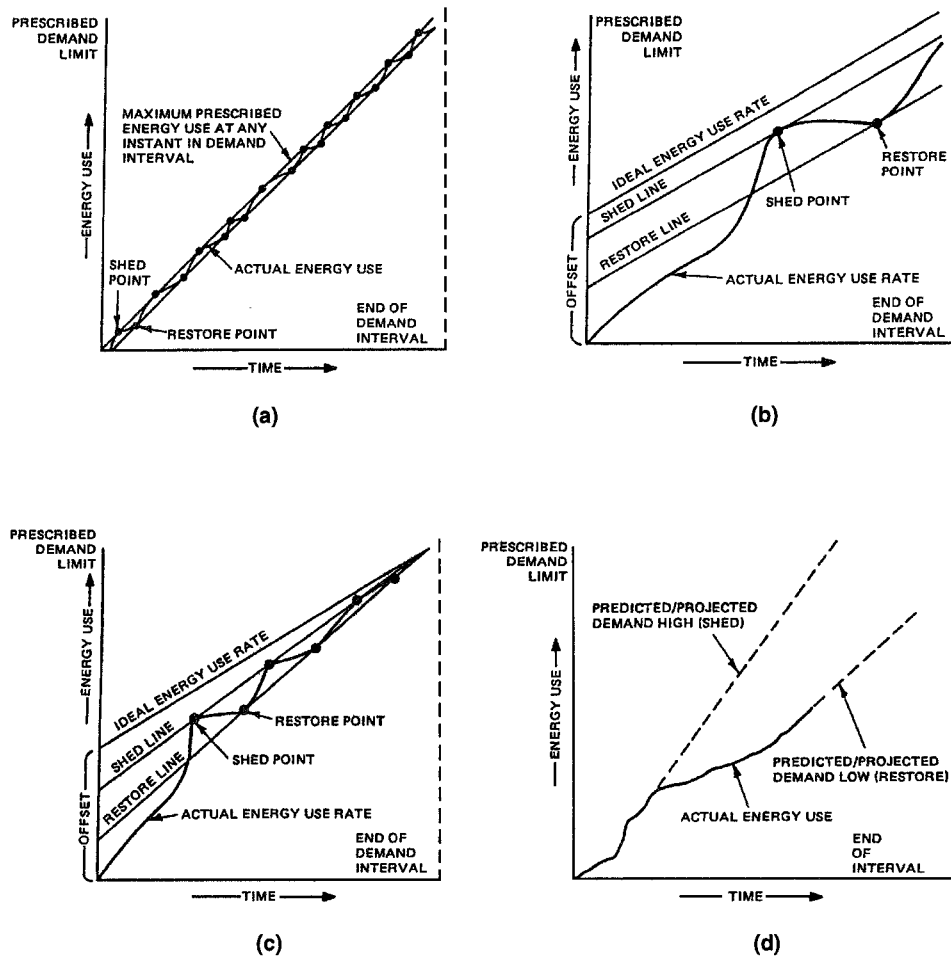
Figure 4-1—Automatic demand control principles (a) Instantaneous demand principle (b) Ideal rate principle (c) Converging rate principle (d) Predicted demand principle (e) Continuous integral principle
