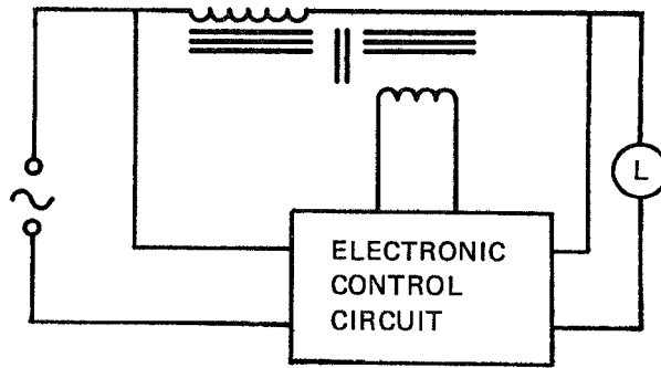
Figure 7-5—Energy-efficient electronically controlled ballast
