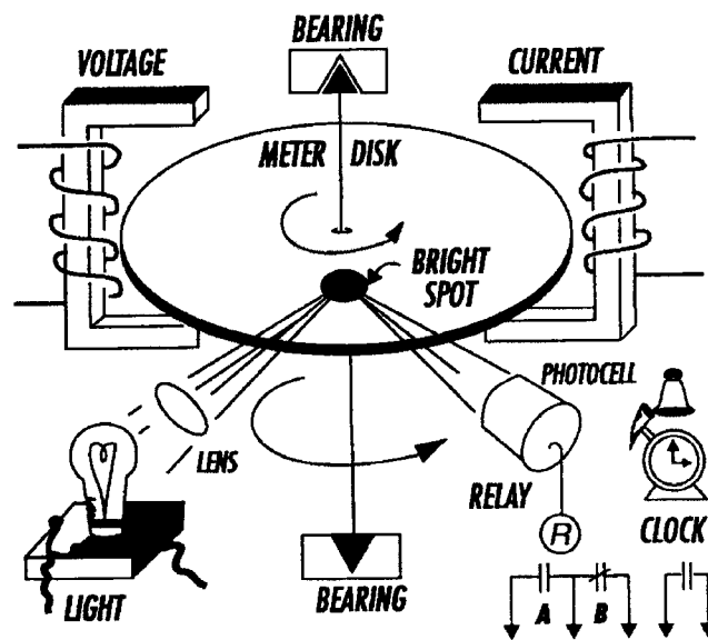
Figure 6-3—Simplified watt-hour meter
