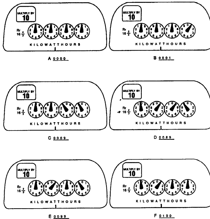
Figure 6-8—kilowatt-hour meter readings
