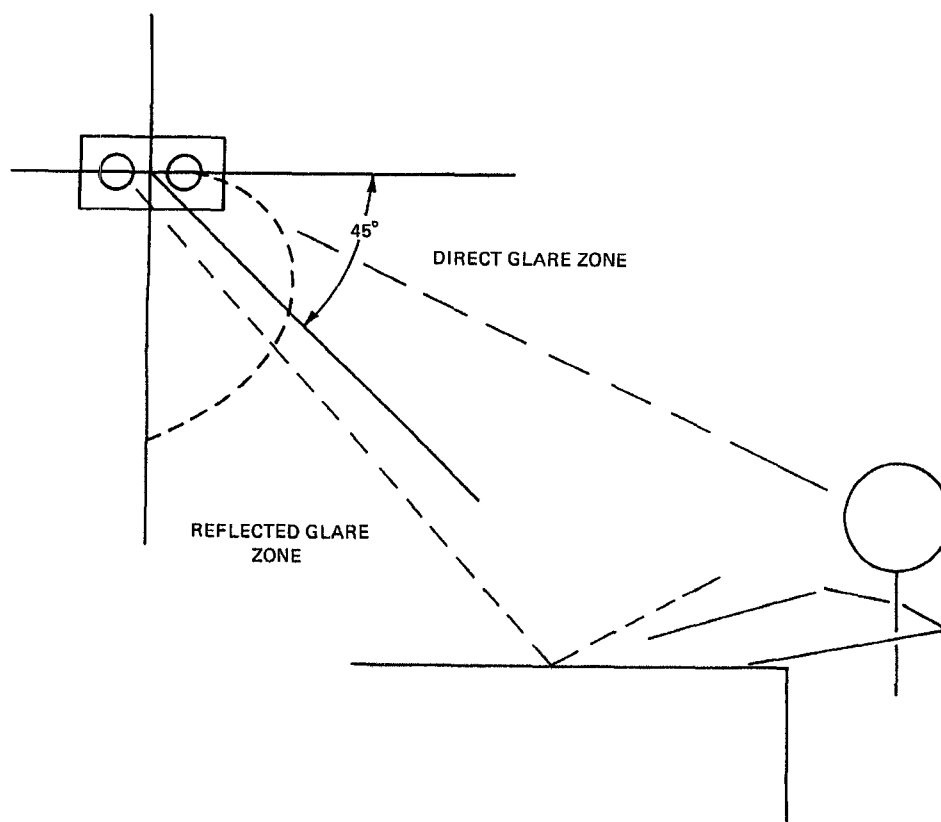
Figure 7-7—Glare illustration
